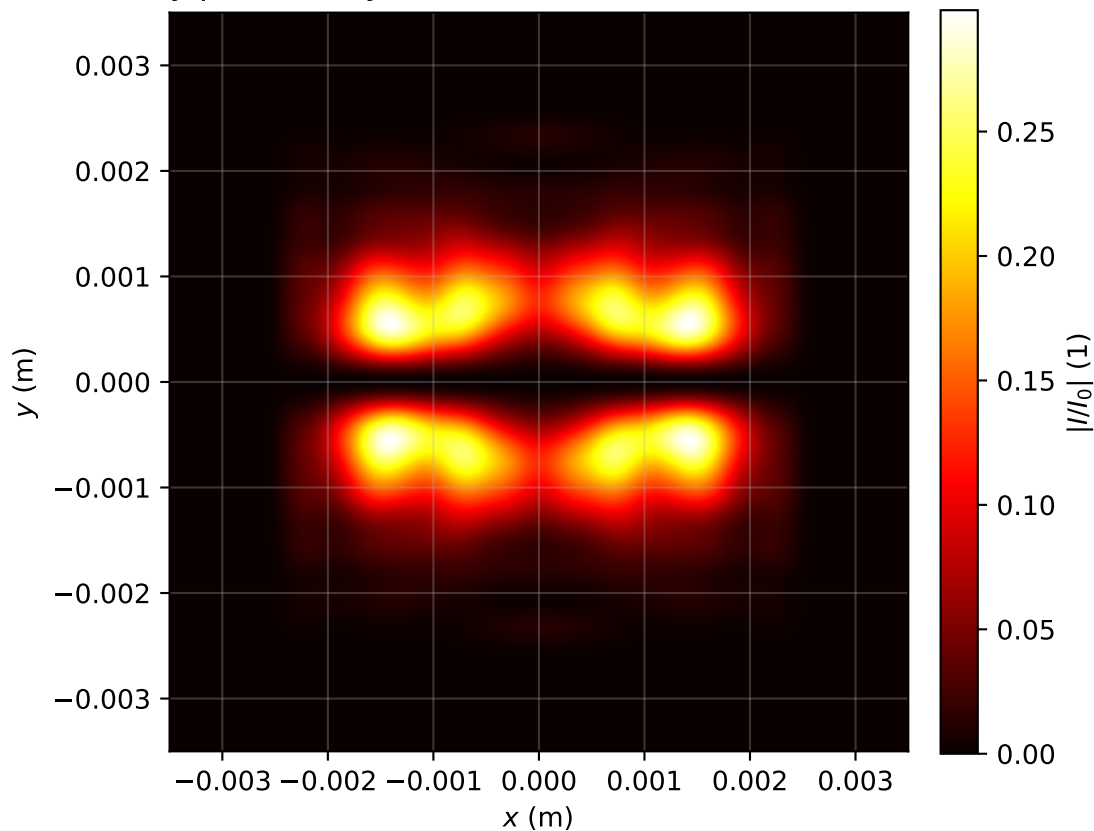
Intensity profile I(x, y, z = 3.344)/I_0 , P_{in}=4.0P_{cr} , artificial time
